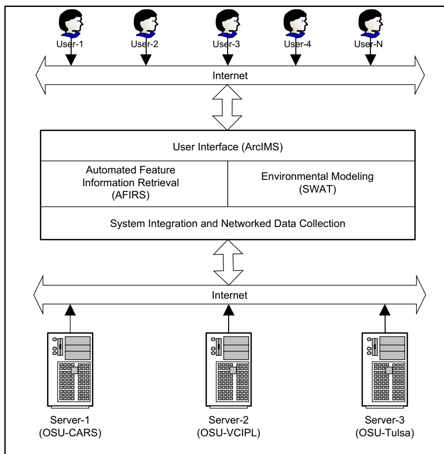
Fig. 1. Integrated system components of the CRP-DSS.
